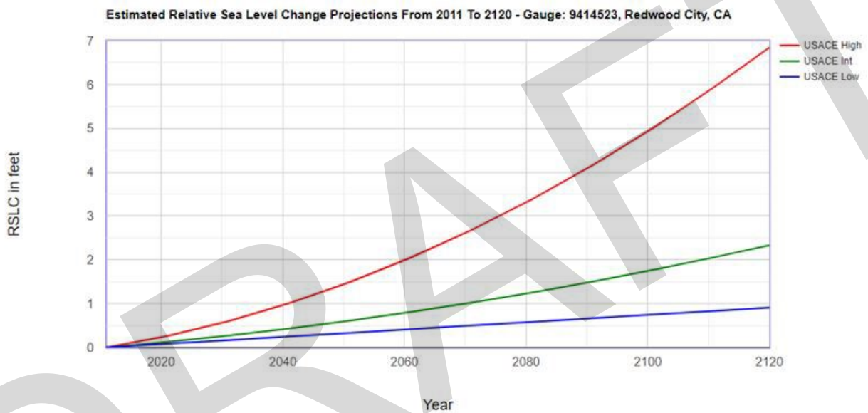
Figure 4. Estimated RLSC projections for NOAA station 9414523 Redwood City, CA
