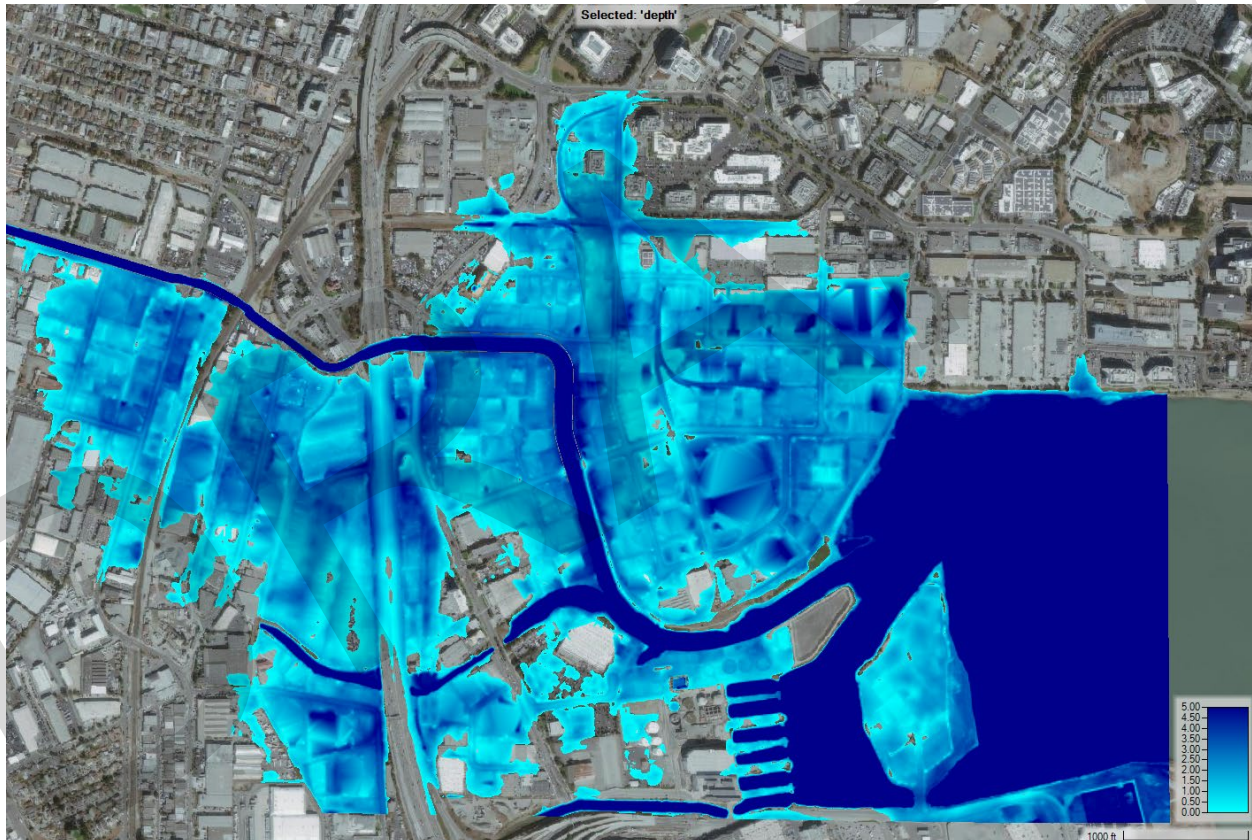
Figure 5. Existing Conditions depth map results for unsteady flow models with 12.99 ft peak tide elevation.
