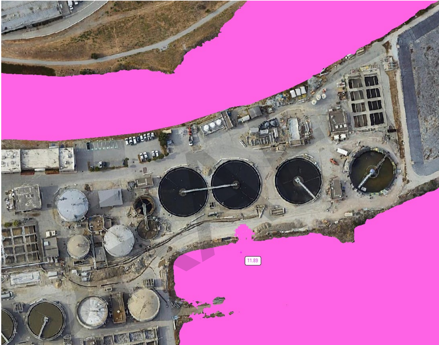
Figure 9. Location of flooding on south side of WQCP area, with North wall in place. Starts at 11.74 ft tide elevation, figure shows 11.89 ft for visualization.
