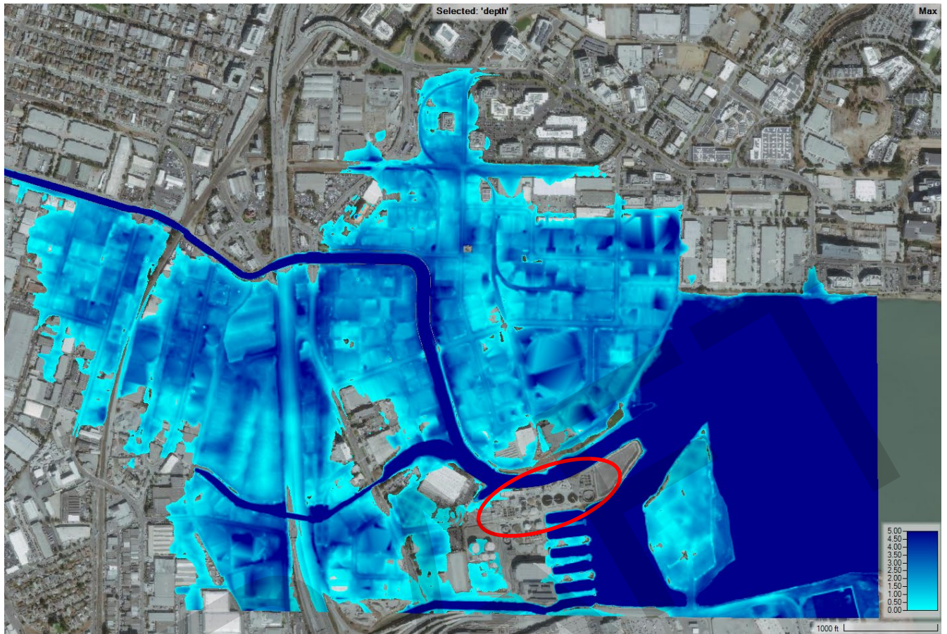
Figure 6. With-Project Alt 2 depth map results for unsteady flow models with 12.99 ft peak tide elevation. Red circle shows WQCP area.
