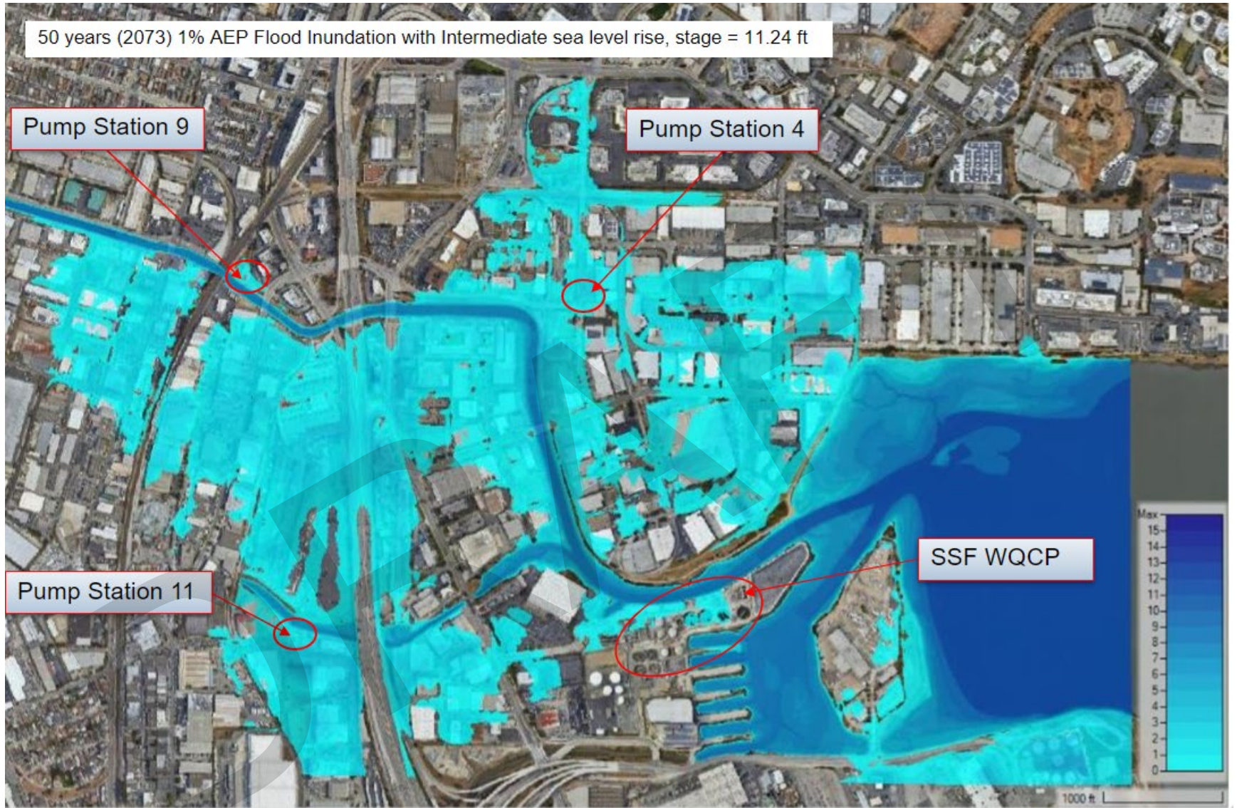
Figure 7. Locations of Pump Stations on 2073, 1% AEP Flood Inundation Map
